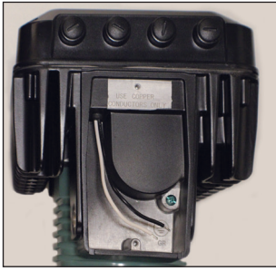
Figure 2 1915ecm Electrical opening: 1/2" 14 MPMSM standard thread
