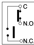
Low water level. Burner off—alarm on.
