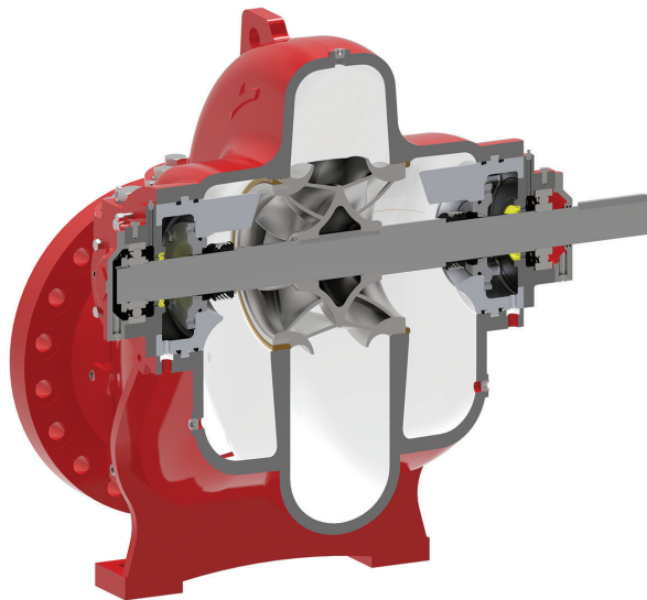
Mechanical Seals Mounted on Shaft
