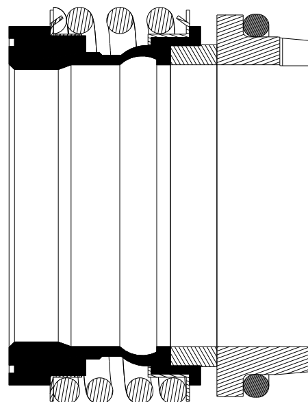
MR2 Metric Rubber Bellow Seal Cross-section
