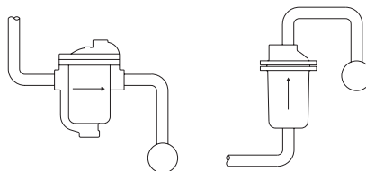
Fig. 2-5. Traps installed with short, well pitched discharge lines to prevent freezups.
